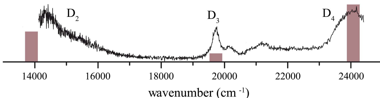
Fig. 2 Photofragmentation spectrum of argon-tagged 1H-phenylene radical cation, compared with the calculated X-MCQDPT2[9,8]/tzv(2df,p) stick spectrum, shifted by +1200\text{ cm}^{-1} . The increased noise at the low-energy end of the spectrum is an artefact of OPO power-correction.
