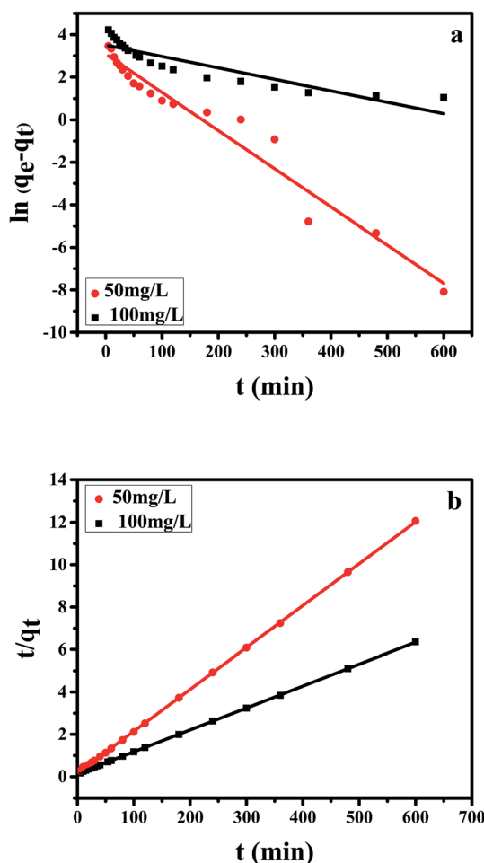
Fig. 4 The (a) pseudo-first-order, (b) pseudo-second-order kinetic model of Cr(vi) removal on the CPA-2.
