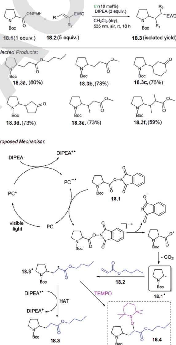
Scheme 18 Decarboxylative alkylation.
