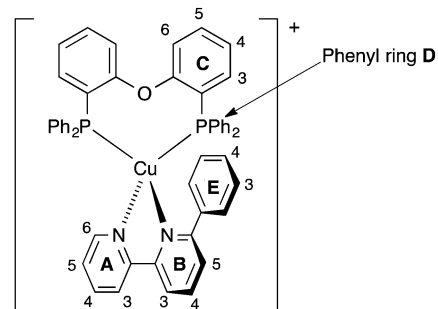
Scheme 2 Atom labelling in [\text{Cu}(\text{POP})(\text{Phbpy})]^\dagger for NMR spectroscopic assignments. Analogous labelling is used for all [\text{Cu}(\text{P}^\wedge\text{P})(\text{N}^\wedge\text{N})]^\dagger complexes.
