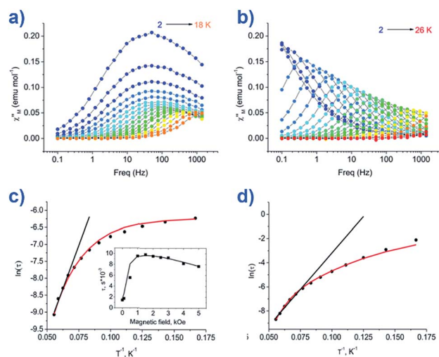
Fig. 14 Out-of-phase magnetic susceptibility for [Co(Pzox) 3 (BC 6 H 5 )Cl] (20) measured under; (a) zero applied dc field and (b) an applied dc field of 1500 Oe. (c) Arrhenius plot of the natural log of the relaxation time vs. inverse temperature under a zero applied dc field and (d) an applied dc field of 1500 Oe. Reprinted with permission from ref. 43. Copyright (2015) American Chemical Society.
