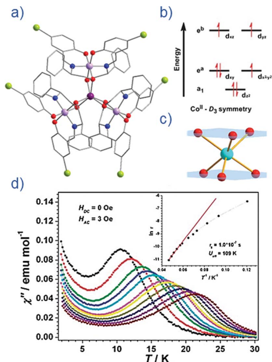
Fig. 13 (a) Molecular structure of [HNEt 3 ][Co II Co III 3 L 6 ] (19). Colour code: dark purple (Co III ), light purple (Co II ), red (O), blue (N), grey (C) and light green (Br). Hydrogen atoms omitted for clarity. (b) Simplified d-orbital splitting diagram (c) simplified coordination environment of central Co II ion and (d) Out-of-phase magnetic susceptibility for 19 under zero applied dc field. Arrhenius plot of natural log of the relaxation time vs. inverse temperature as inset. Reprinted with permission from ref. 42. Copyright (2013) Royal Society of Chemistry.
