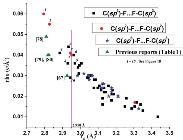
Fig. 17 Comparison of the variation of the electron density ( \text{e} \text{ Å}^{-3} ) at the BCP and with the F...F bond path length (Å) for C(sp 3 )/(sp 2 )–F...F–C(sp 3 )/(sp 2 ) interactions from current and previous studies [total 64 data points].
