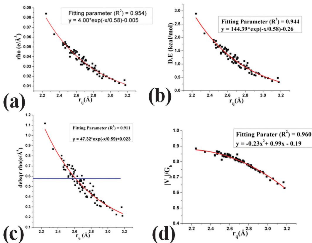
Fig. 14 Variation of (a) electron density (e Å -3 ) at the BCP, (b) dissociation energy (D.E.) (kcal mol -1 ) with the H...F bond path length (Å), (c) Laplacian ( \nabla^2\rho ) at the BCP and (d) |V_b|/G_b with the H...F bond path length (Å).
