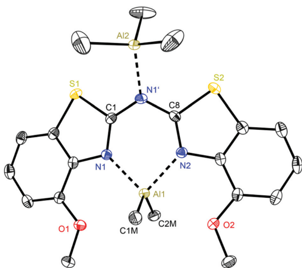
Fig. 7 Molecular structure of [\text{Me}_2\text{Al}(\{4\text{-OMeNCSC}_6\text{H}_3\}_2\text{N})\cdot\text{AlMe}_3] ( 6 ). Anisotropic displacement parameters are depicted at the 50% probability level. Co-crystallised solvent molecules, hydrogen atoms and positional disorder of the whole molecule are omitted for clarity. Structural data are given in Tables 1 and 3.
