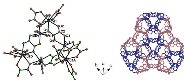
Fig. 26 Left: Representation of the 3D anionic network of \{(\text{NH}_2\text{Me}_2)_2[\text{Cd}_3(\text{C}_2\text{O}_4)_4] \cdot \text{MeOH} \cdot 2\text{H}_2\text{O}\}_n ; right: representation of the hexanuclear octupolar structure of [\text{Cd}_6(\text{C}_2\text{O}_4)_8]^{4-} . Adapted from ref. 113 (Copyright © 2007 John Wiley & Sons).
