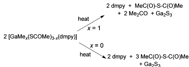
Scheme 2 Decomposition of [GaMe(SCOMe) 2 (dmpy)] and [Ga(SCOMe) 3 (dmpy)].
