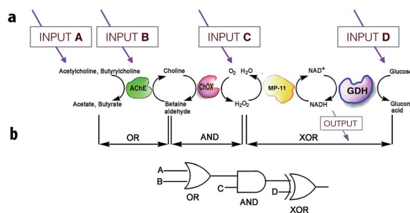
Fig. 5 Scheme illustrating the operation of concatenated logic gates based on four coupled enzyme systems. (a) Cascade of reactions catalyzed by AChE, ChOx, MP-11, and the NAD + -dependent GDH; all triggered by input signals that include acetylcholine, butyrylcholine, O 2 , and glucose added in different combinations. (b) Network performing OR-AND-XOR operations. Adapted with permission from ref. 30. Copyright (2006) National Academy of Sciences, U.S.A.
