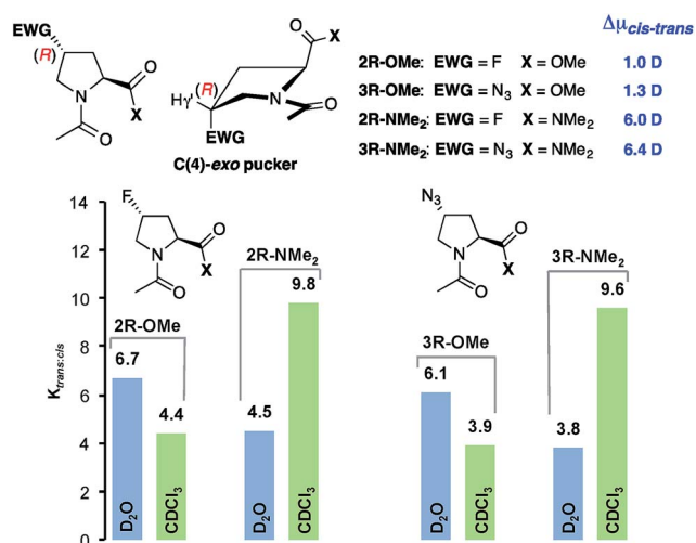
Fig. 5 K_{\text{trans/cis}} values of (4 R )-configured Ac-Xaa-OMe and Ac-Xaa-NMe 2 of Fip and Azp derivatives determined by NMR-spectroscopy of 80 mM solutions in \text{D}_2\text{O} (blue) and \text{CDCl}_3 (green) and difference in the dipole moments ( \Delta\mu_{\text{cis-trans}} ) of trans and cis conformers calculated with \text{CHCl}_3 as solvent at the PBE0-D3-COSMO/def2-TZVP level of theory.
