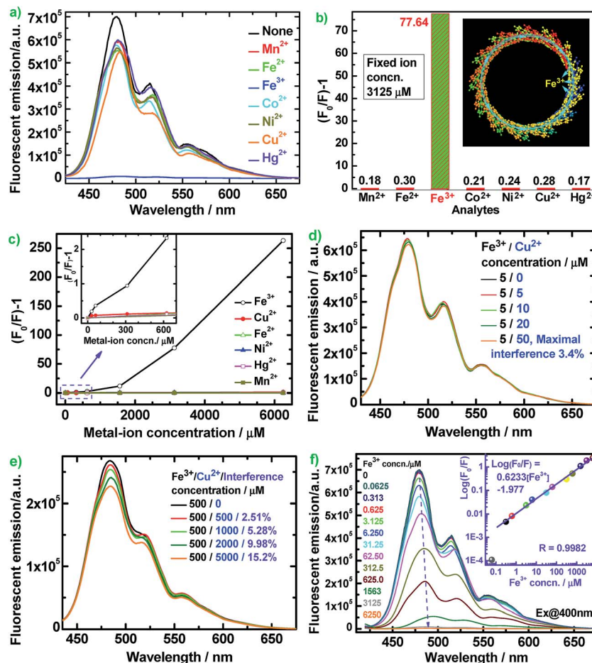
Fig. 8 (a) Fluorescence emission spectra and (b) (F_0/F) - 1 values of 10 \text{ mg L}^{-1} optimal PFA in DMSO containing different metal ions at a fixed concentration of 3125 \text{ }\mu\text{M} (inset: schematic diagram of the amplified quenching of PFA fluorescence by \text{Fe}^{3+} ); (c) relationship between (F_0/F) - 1 and metal-ion concentration of 10 \text{ mg L}^{-1} optimal PFA in DMSO; (d and e) the influence of coexisted \text{Cu}^{2+} on the PL emission of the optimal PFA solution containing \text{Fe}^{3+} ; (f) PL emission spectra of 10 \text{ mg L}^{-1} optimal PFA in DMSO containing \text{Fe}^{3+} of 0 to 6250 \text{ }\mu\text{M} .
