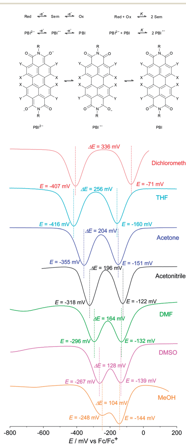
Fig. 3 Top: schematic representation of the equilibrium between reduced form (Red \rightleftharpoons Sem \rightleftharpoons Ox), intermediate (Sem \rightleftharpoons PBI ^{\cdot-} ) and fully oxidized form (Ox \rightleftharpoons PBI). Bottom: square wave voltammograms of PBI 3 in solvents of different polarity. The dianion disodium salt 4 was used in the case of MeOH for solubility reasons. Reference electrode: Ag/AgCl, working and auxiliary electrode: Pt; 0.1 M TBAHFP, \text{Fc}/\text{Fc}^+ , 25 °C, c \sim 2 \times 10^{-4} M.
