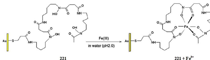
Fig. 185 Schematic of the proposed mechanism for the Au-MSA-DFO SAM 221 formation and its interaction with \text{Fe}(\text{III}) .
