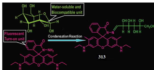
Fig. 275 Chemical structure of ligand 313 .
