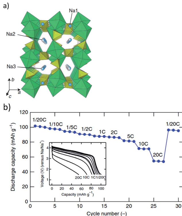
Fig. 8 (a) \text{Na}_2\text{Fe}_2(\text{SO}_4)_3 structure projected along the c axis, and (b) capacity retention upon cycling up to 30 cycles under various rate of C/20 (2 Na in 20 h) to 20 C. Reproduced with permission 80 © 2014, Nature Publishing Group.
