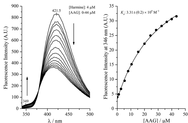
Fig. 1 Emission spectra of harmine measured in AAG solution at increasing protein/ligand molar ratios (2 mL of harmine solution was titrated with 200 \mu\text{M} AAG dissolved in the ligand solution). Fluorescence intensities plotted against the AAG concentration of the sample solution. The solid line is the result of non-linear fitting analysis.
