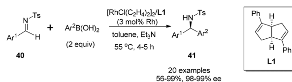
Scheme 18 Catalytic asymmetric arylation of aryl N -tosyl imines with arylboronic acids.
