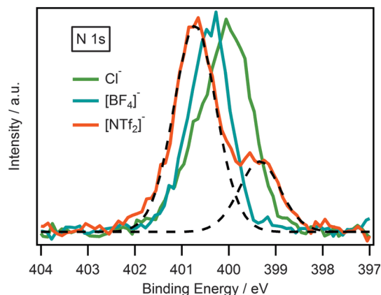
Fig. 5 N 1s XPS spectra of [(C_8C_1)_2dmg][NTf_2] , [(C_8C_1)_2dmg][BF_4] and [(C_8C_1)_2dmg][Cl] . Intensities are normalised to the N_{cation} 1s peak for [(C_8C_1)_2dmg][BF_4] . XPS spectra were charge corrected by referencing the aliphatic C 1s photoemission peak to 285.0 eV. Deconstruction of the N 1s XPS photoemission peaks (dotted line) for the [(C_8C_1)_2dmg][NTf_2] highlighting the two nitrogen components, N_{cation} at higher binding energy and N_{anion} at lower binding energy.
