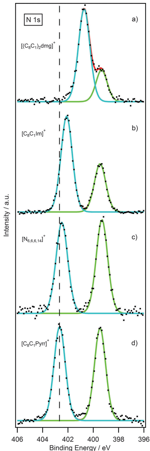
Fig. 6 N 1s XP spectra of (a) [(C_8C_1)_2dmg][NTf_2]^+ , (b) [C_8C_1Im][NTf_2]^+ , (c) [N_{6,6,6,14}][NTf_2]^+ and (d) [C_8C_1Pyr][NTf_2]^+ . Intensities are normalised to the F 1s peak for [C_8C_1Pyr][NTf_2]^+ . XP spectra were charge corrected by referencing the aliphatic C 1s photoemission peak to 285 eV.
