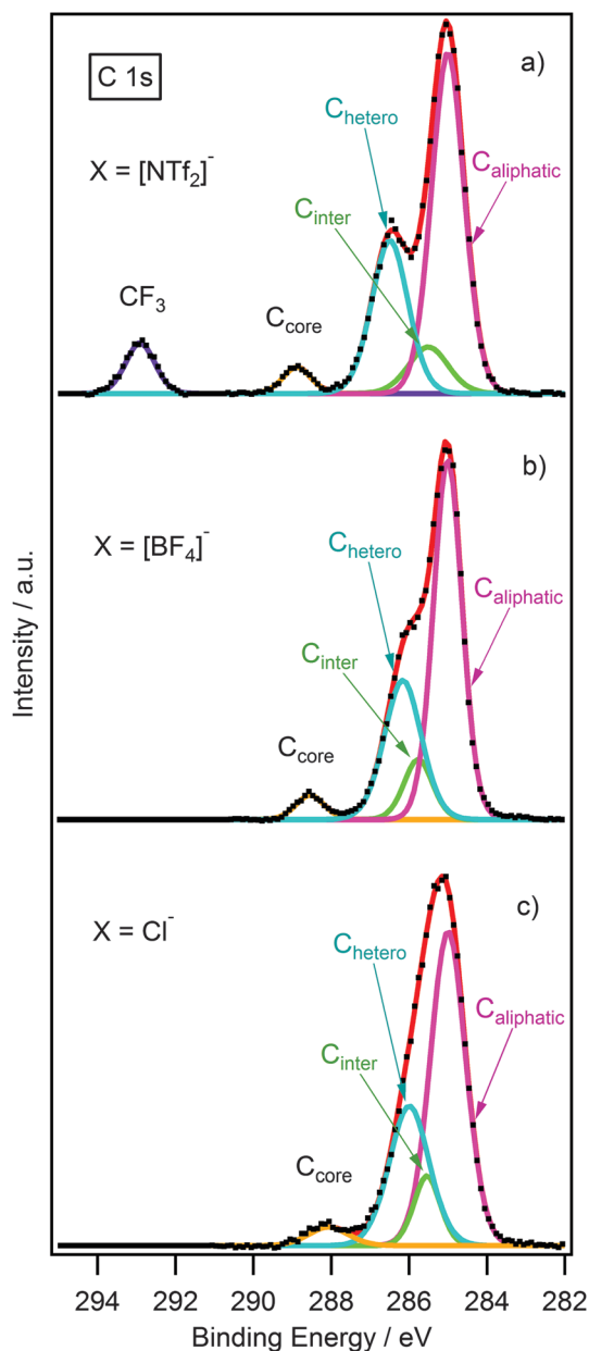
Fig. 4 High resolution XPS spectra of the C 1s region with component fittings for (a) [(C_8C_1)_2dmg][NTf_2] , (b) [(C_8C_1)_2dmg][BF_4] and (c) [(C_8C_1)_2dmg][Cl] . Intensities are normalised to the N_{cation} 1s photoemission peak for [(C_8C_1)_2dmg][BF_4] . All XPS spectra charge corrected to C_{aliphatic} = 285.0 eV.
