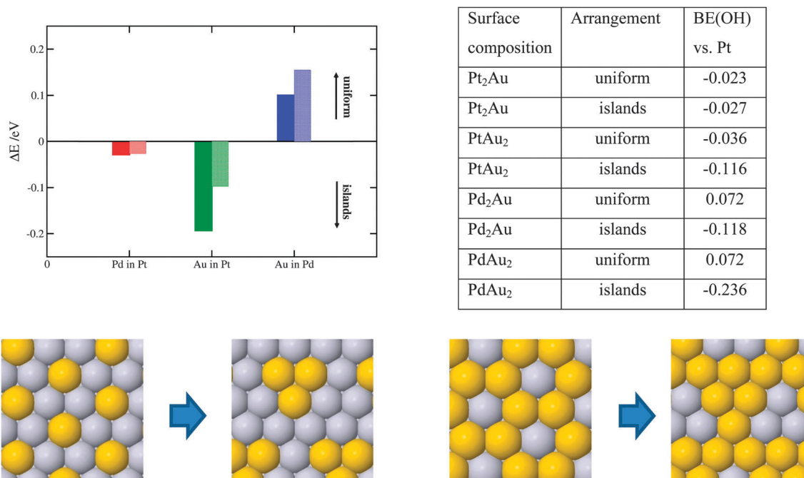
Fig. 5 The plot shows the energy difference between the uniform and cluster arrangement of solute atoms in the surface layer as illustrated below. Solid and transparent columns are for 1/3 ML and 2/3 ML surface solute concentration, respectively. The tabulated values show the changes in the OH BE for the two extremes for PtAu and PdAu thin films. Values are given in eVs. The reference value is +0.1 eV relative to Pt that corresponds to the OH BE at the top of the volcano.
