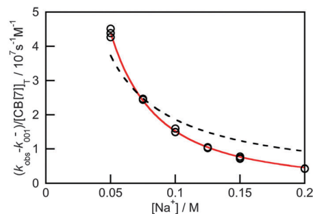
Fig. 4 Dependence of the overall association rate constant with the concentration of \text{Na}^+ . The red solid line corresponds to the fit of the data to eqn (9), which assumes that two sodium cations are bound to CB[7]. The dashed line corresponds to the best fit when the binding of only one sodium cation to CB[7] is assumed. (Reprinted with permission from H. Tang, D. Fuentealba, Y. H. Ko, N. Selvapalam, K. Kim and C. Bohne, J. Am. Chem. Soc. , 2011, 133 , 20623–20633. Copyright 2011 American Chemical Society.)
