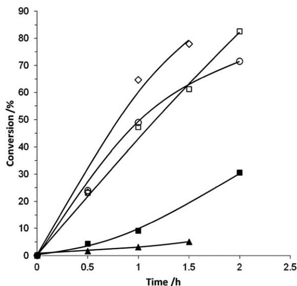
Fig. 1 The conversion of benzyl alcohol by catalysts prepared using various preparation techniques: \blacktriangle Au/ \text{TiO}_2 (PG), \blacksquare AuPd/ \text{TiO}_2 (IMP), \circ AuPd/ \text{TiO}_2 (DP), \square AuPd/ \text{TiO}_2 (PG), \diamond Pd/ \text{TiO}_2 (PG).
