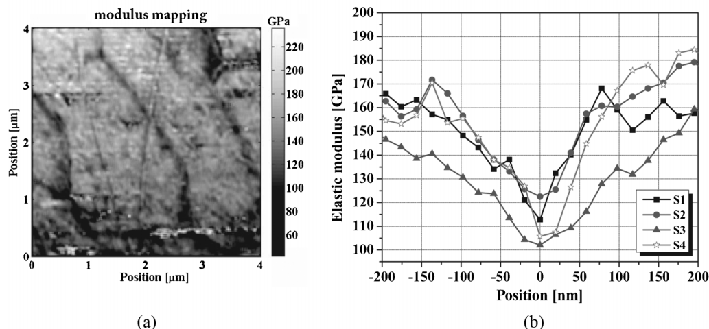
Fig. 18 (a) Map of elastic modulus taken from the nacre layer at a depth of 300\ \mu\text{m} beneath the inner surface of the bivalve shells of Perna canaliculus ; (b) the modulus change across organic–inorganic interfaces. 110
