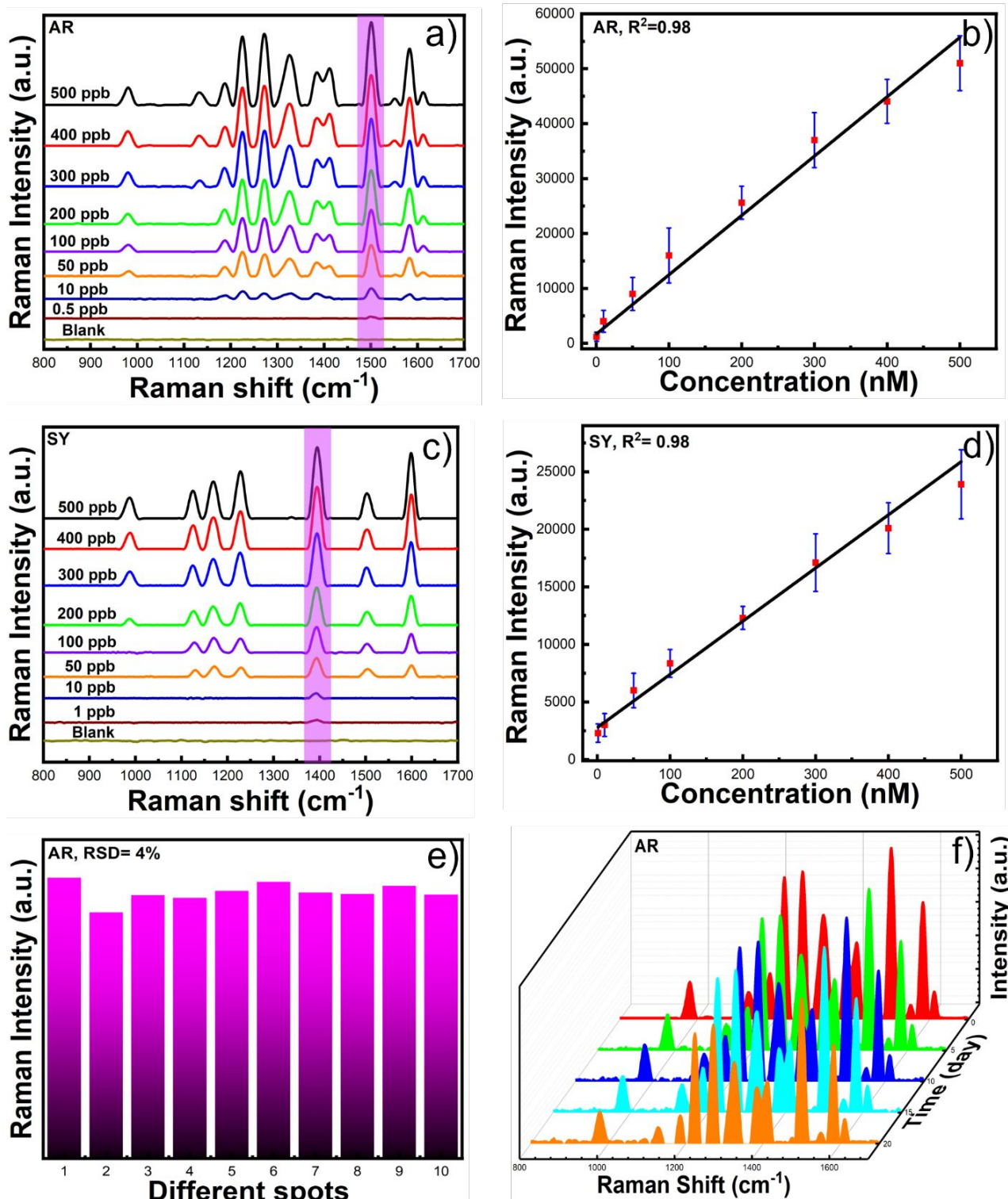
Figure 3. SERS spectra of AR using GNS-5 at different concentrations from 500 ppb to 0.5 ppb (a). The calibration curve for the characteristic peak intensity at 1500 cm -1 as a function of AR concentration (b). SERS spectra of SY at different concentration from 500 ppb to 1 ppb (c) and SERS intensity of SY at 1395 cm -1 as a function of different concentrations (d). SERS reproducibility of allura red using GNS-5 (e). Representative SERS spectra of GNS-5 after 20 days measured with 5 days interval showing good stability of GNS-5(f).
