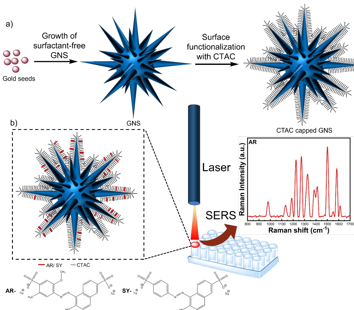
Scheme 1. Schematic of the synthetic procedure of CTAC capped GNS-5 where the GNS-5 morphology was achieved by systematic controlling of the concentrations of reagents including gold salt, HCl, ascorbic acid, and \text{AgNO}_3 (a), and a simple procedure for SERS detection of weak-affinity analytes which involves simple mixing of analytes in a well plate having CTAC capped GNS-5 (b).
