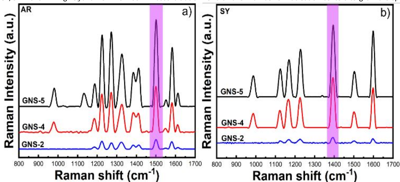
Figure 2. Comparison of SERS signal intensity of allura red dye using GNS-2, GNS-4, and GNS-5 (a). Comparison of SERS signal intensity of sunset yellow with GNS-2, GNS-4, and GNS-5 (b).
