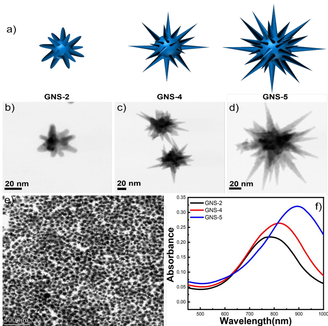
Figure 1. 3D model of GNS-2, GNS-4, and GNS-5 morphology (a). TEM image of GNS-2 (b), GNS-4 (c) and GNS-5 (d). TEM image having multiple nanostars of GNS-5 showing high monodispersity of the synthesis (e). UV-vis spectra of GNS-2, GNS-4, and GNS-5 morphology showing a red shift from 780 nm to 890 nm when the GNS morphology changes from GNS-2 to GNS-5 (f).
