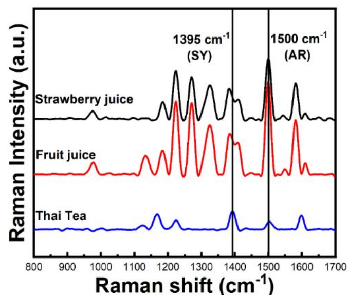
Figure 4. Representative SERS spectra of beverages where GNS-5 was utilized as a SERS probe.
