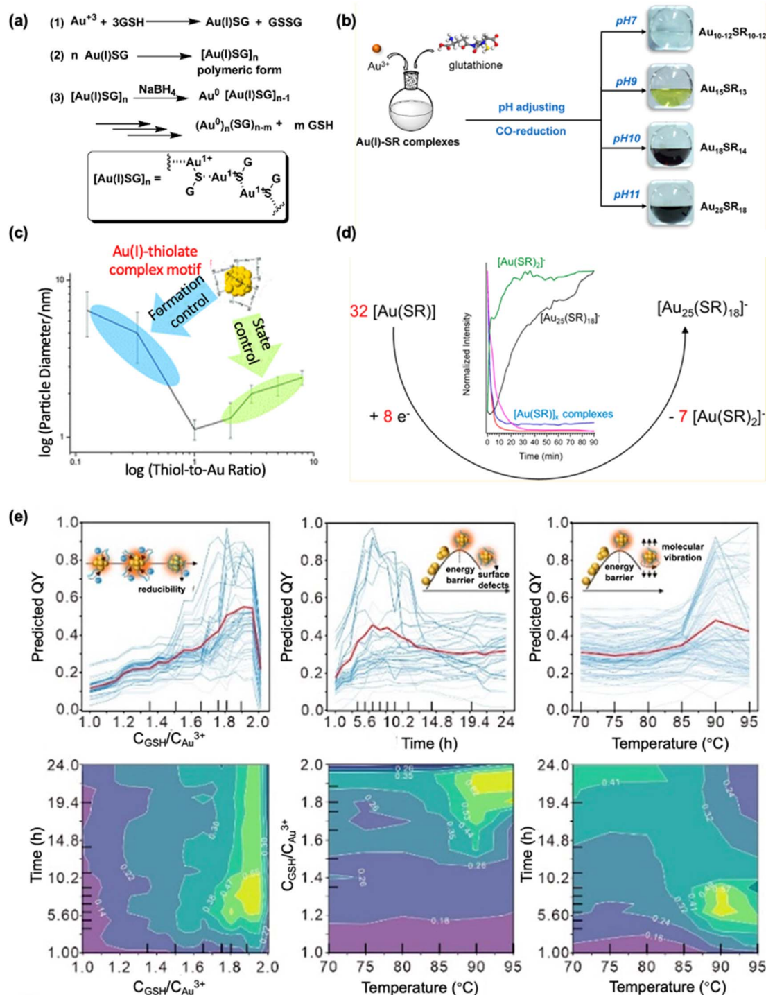
Fig. 3 Dual roles of GSH and parameter space in the Brust–Schiffrin method. (a) Proposed mechanism for the formation of Au NPs from Au 3+ and GSH. Reprinted with permission from ref. 66. Copyright 2008 American Chemical Society. (b) Schematic illustration depicting the production of Au 10-12 , Au 15 , Au 18 , and Au 25 NCs by adjusting the pH of the reaction solution in the CO-reduction method. Reprinted with permission from ref. 25. Copyright 2013 American Chemical Society. (c) A U-shape trend is identified between the size of Au NPs and the thiol-to-Au ratio. Reprinted with permission from ref. 89. Copyright 2016 Royal Society of Chemistry. (d) Synthesis of water-soluble Au 25 (SR) 18 using a stoichiometric amount of NaBH 4 . Reprinted with permission from ref. 90. Copyright 2018 American Chemical Society. (e) Explainability of machine learning studies of complex correlations among synthetic parameters for GSH-protected Au NCs. Reprinted with permission from ref. 91. Copyright 2023 Royal Society of Chemistry.
