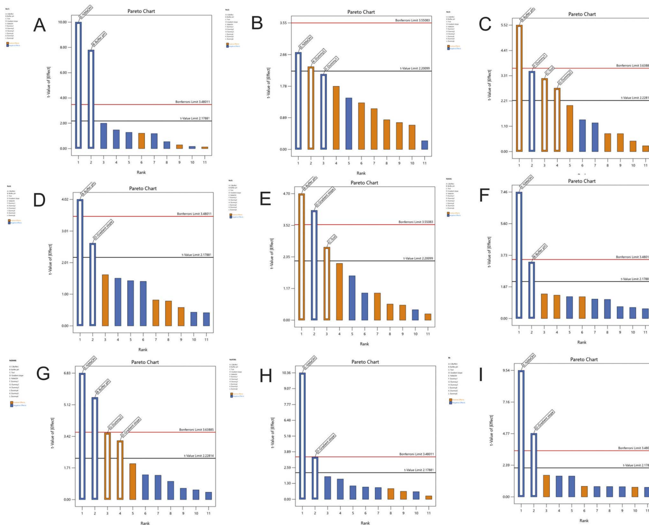
Fig. 2 Pareto charts for the chromatographic parameters: (A) R_{s(1)} , (B) R_{s(2)} , (C) R_{s(3)} , (D) R_{s(4)} , (E) R_{s(5)} , (F) N_{ASA} , (G) N_{RAM} , (H) N_{ATOM} and (I) R_t .
