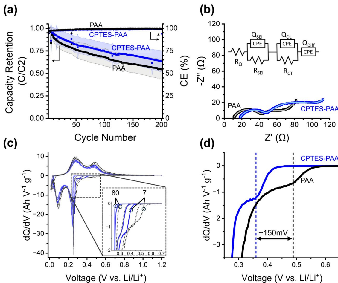
Fig. 3. (a) Cycling performance for PAA and CPTES-PAA cells. On the left y-axis is silicon lithiation capacity retention (relative to the second cycle) of half-cells made using PAA (black) or CPTES-PAA (blue) binder. Shaded areas indicate error of 1 standard deviation. This data is the average over many cells cycled a different number of times: with 30/33 cells at cycle 1, 16/17 at cycle 100, and 10/13 at cycle 200 for PAA /CPTES-PAA cells (see Fig. S1). On the right y-axis is coulombic efficiency (CE, ratio between lithiation and delithiation capacity). (b) Nyquist plot from half-cells after seven cycles using PAA (OCP before scan: 0.237 V) or CPTES-PAA (OCP before scan: 0.238 V) electrodes, the equivalent circuit model, and the equivalent circuit model fits (lighter colored lines). (c) Differential capacity ( dQ/dV ) of selected initial cycles (7, 15, 50, 80 from darker to lighter) for half-cells. PAA cells are black/grey dashed traces, CPTES-PAA cells are solid blue traces. (d) Magnification of dQ/dV of 7 th cycle in pre-alloying potential range, showing overpotential for the shoulder. Vertical lines are provided as guides to the eye.
