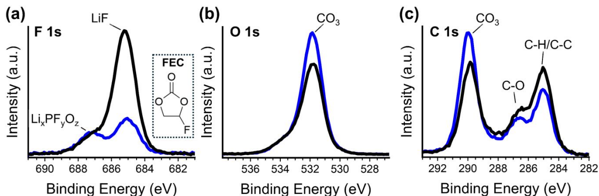
Fig. 6. F 1s (a), O 1s (b), and C 1s (c) XPS spectra of 7 cycled PAA (black) and CPTES-PAA (blue) electrodes. Structure of fluoroethylene carbonate is shown in inset in (a).
