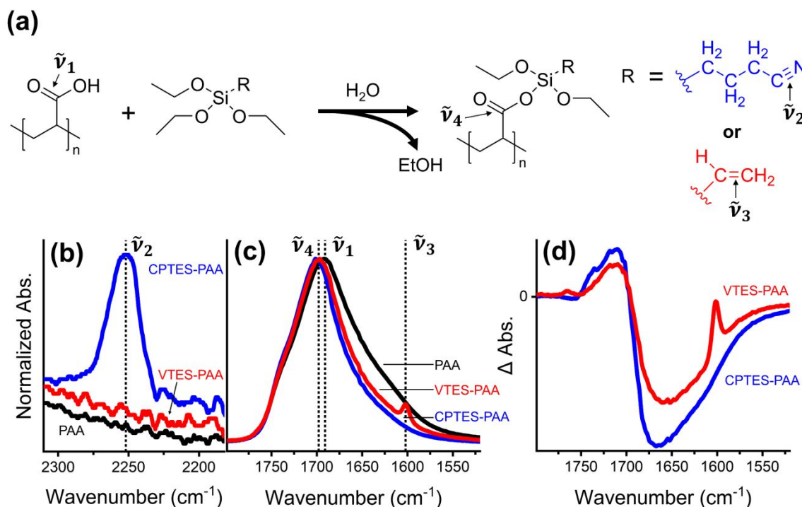
Fig. 2. (a) Reaction scheme of polyacrylic acid (PAA) with either 3-cyanopropyltriethoxysilane (CPTES) or vinyltriethoxysilane (VTES). Normalized (to the carbonyl stretch [between 1690 cm -1 and 1702 cm -1 ]) FTIR spectra of: nitrile stretch, \tilde{\nu}_2 , (b), vinyl stretch, \tilde{\nu}_3 , carboxylic acid carbonyl stretch, \tilde{\nu}_1 , and silyl ester carbonyl stretch, \tilde{\nu}_4 (c). Traces in (d) are difference spectra of modified binders minus PAA binder. For all plots, black traces correspond to PAA binder, blue to CPTES-PAA, and red to VTES-PAA.
