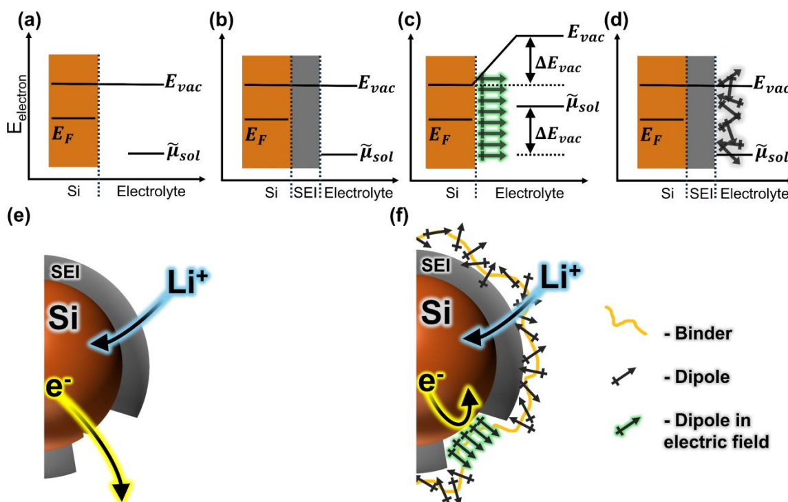
Fig. 1. Plots (a-d) illustrate the electronic energetics at the SEI (grey) vs. the defect sites with and without dipoles. Cartoons show a silicon particle (brown) without (e) and with (f) a layer of conformationally labile dipoles (black crossed arrows). Without a dipolar layer (e), there is little electric field at the surface of the SEI due to the ionic gradient across the SEI (b). At the defects, however, the field is large (a). Lithium-ions (blue) may traverse the SEI (b and e), but electrons (yellow) may not (curved arrows indicate movement of charge). At defect sites, either charged species may move between the electrolyte and the silicon (a and e). With a layer of conformationally labile dipoles (f), the field at the defects imparts a preferred orientation of the dipoles. This layer of aligned dipoles causes a shift in the vacuum level ( E_{vac} ) and the electrochemical potential ( \tilde{\mu}_{sol} ) across this interface, modulating the kinetics of charge transport across it (c and f). At the SEI interface with a layer of conformationally labile dipoles, however, there is little field, and therefore no preferred orientation for the dipoles (d and f). This leaves the vacuum level, and thus the charge transfer kinetics, unchanged from the no-dipole case (b).
