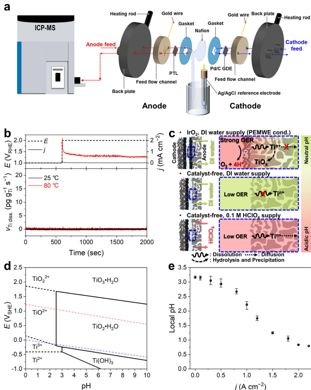
Fig. 1 (a) Schematic representation of the online PEMWE/ICP-MS setup. (b) Real-time Ti dissolution measured at a static potential of 2 V_{\text{RHE}} with a supply of \text{O}_2 -saturated DI water at 25 and 80 °C. (c) Schematic representation of Ti dissolution behavior under three different operating conditions: PEMWE operation (i.e., Ti PTL with a catalyst layer and DI water supply) and our model systems of catalyst-free Ti PTLs with DI water or 0.1 M \text{HClO}_4 supply. (d) Pourbaix diagram of Ti. (e) Estimated local pHs at the electrode–membrane interface measured at different current densities.
