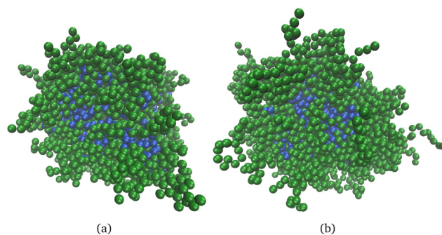
Fig. 2 Snapshots of neutral core-shell nanogels. The core particles are blue; the green particles belong to the nanogel shell. The total number of particles in the shell is N^{\text{sh}} = 2000 : (a) M_{\text{sh}} = 10 , K_{\text{sh}} = 200 ; (b) M_{\text{sh}} = 20 , K_{\text{sh}} = 100 . The shell of the nanogels is non-cross-linked.
