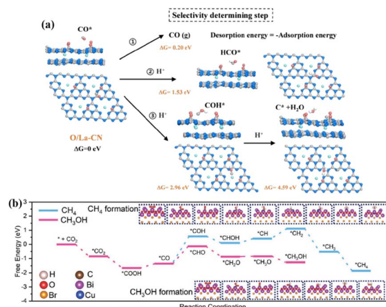
Fig. 7 (a) Calculated free energy for the photocatalytic CO 2 reduction reaction of the selectivity-determining step. This figure has been reproduced from ref. 67 with permission from American Chemical Society, copyright 2020. (b) The DFT-calculated free energy diagram for the hydrogenation of CO 2 to CH 3 OH and CH 4 over Cu 1 @BiOBr. This figure has been reproduced from ref. 68 with permission from Wiley-VCH, copyright 2023.
