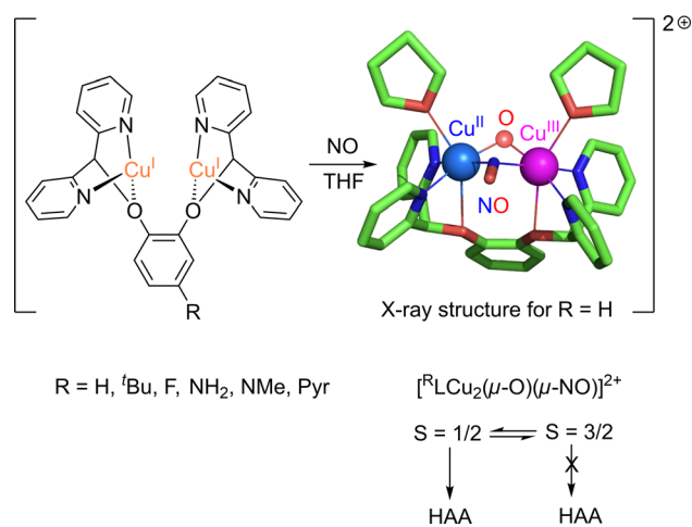
Fig. 10 Synthesis of [\text{R}]\text{LCu}_2(\mu\text{-O})(\mu\text{-NO})]^{2+} species and influence of the spin state on HAA reactivity from ref. 73 and 74.
