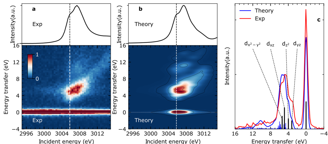
Fig. 2 VtC-RIXS of CpRh(CO) 2 as a probe of MC d–d final states. (a) Experimental Rh L-edge X-ray absorption spectrum (top) and Rh L-edge RIXS map (bottom) for CpRh(CO) 2 . (b) Simulated Rh L-edge X-ray absorption spectra and RIXS map at the TD-DFT level of theory. X-ray absorption spectra result from integration of RIXS intensities in a given incident-energy range along the energy-transfer axis. Vertical dashed lines in (a) and (b) indicate the energy of 3005.8 eV at which cuts were obtained to target the valence-excited MC states or, alternatively, HOMO, HOMO–1, to LUMO transitions. (c) Cuts from the experimental and simulated RIXS maps at 3005.8 eV. The dominant peaks correspond to transitions from the ground to MC states or, alternatively, to the HOMO, HOMO–1, HOMO–2, HOMO–3 ( 4d_{yz} , 4d_{z^2} , 4d_{xz} , and 4d_{x^2-y^2} , respectively) to 4d_{xy} LUMO orbital transitions.
