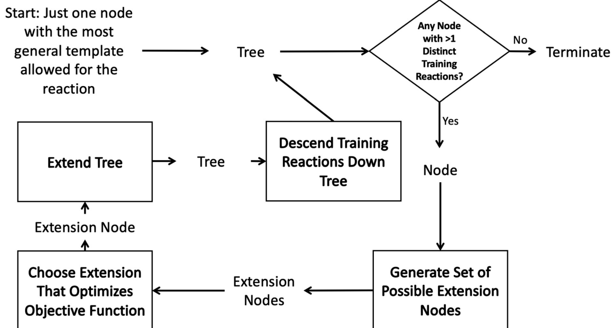
Fig. 2 Decision tree estimator generation algorithm.
