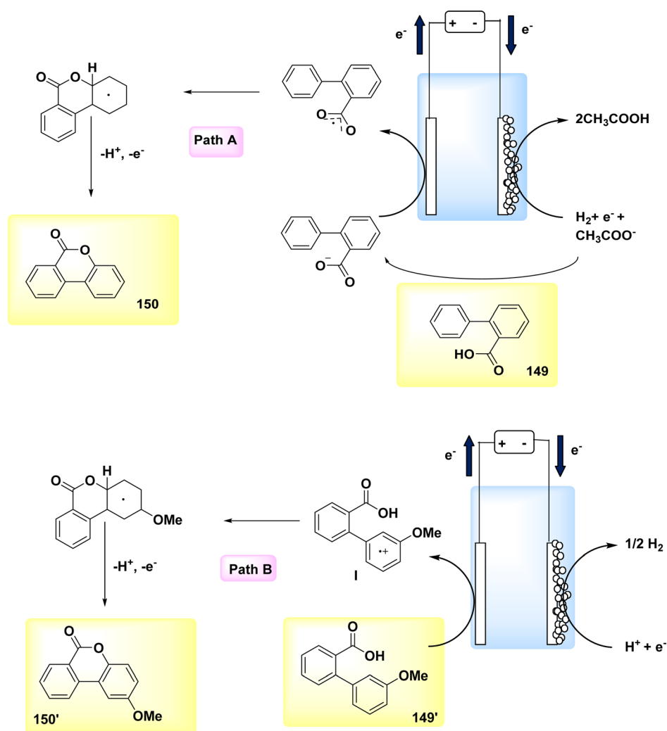
Scheme 57 The electroynthesis of 6 H -benzo[ c ]chromen-6-one 150 and its CH 3 O - derivative 150' with its proposed mechanism.
