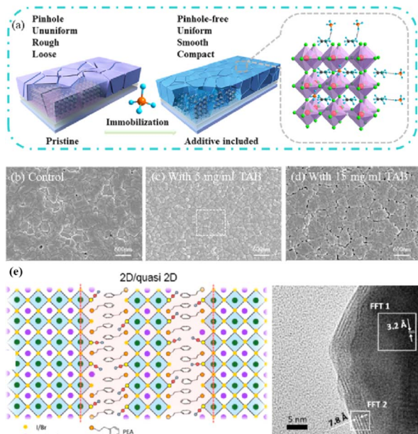
Fig. 26 (a) Schematic demonstration of the process of superhalogen BH 4 - -induced morphological changes of the perovskite film. (b–d) Top-view SEM images of perovskite films with 0, 5, and 15 mg mL -1 tetrabutylammonium borohydride (TAB) additives deposited on mesoporous-TiO 2 /compact TiO 2 /FTO/glass substrates. Adapted with permission from ref. 78. Copyright 2020 American Chemical Society. (e) Formation mechanism and TEM images of the (quasi)-2D/3D structure constructed using PEA and Pb(SCN) 2 as additives. Adapted with permission from ref. 238. Copyright 2019 Elsevier.
