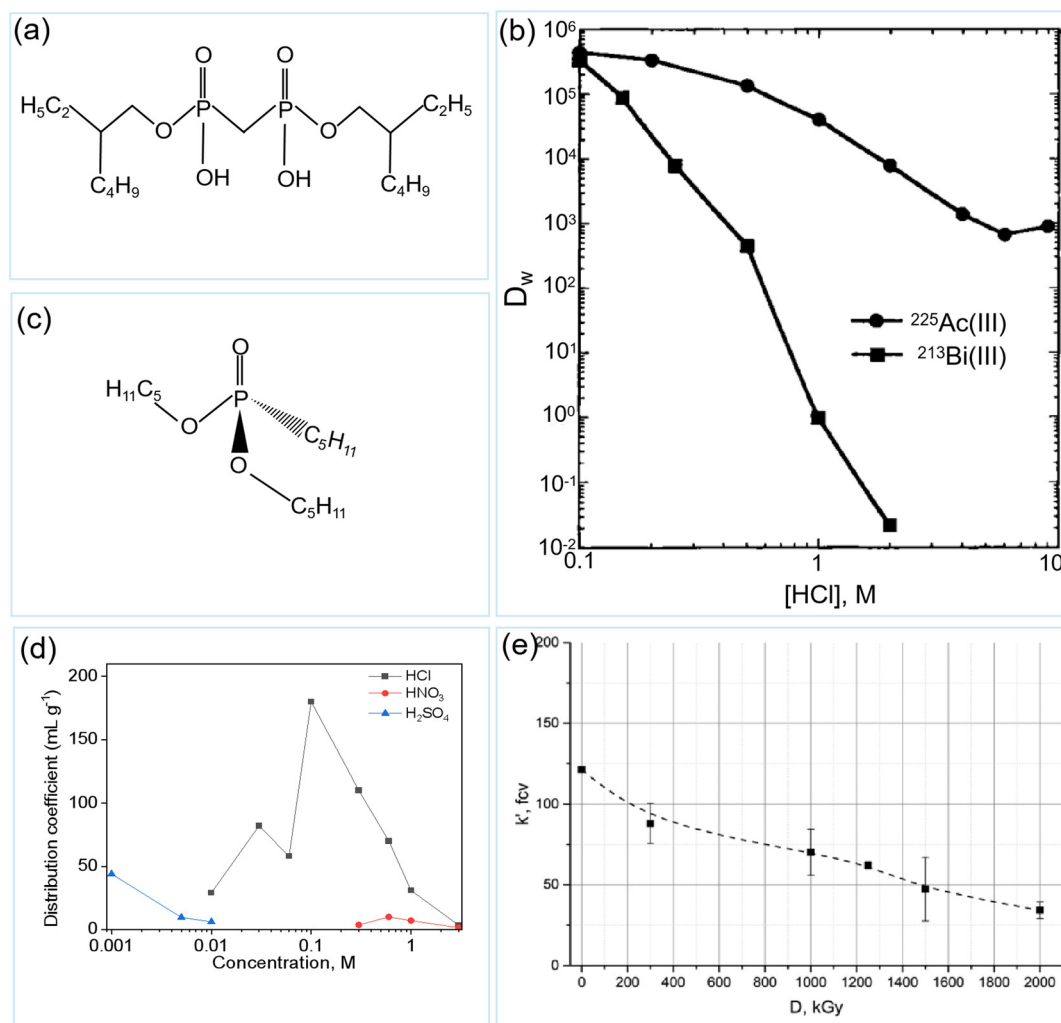
Fig. 15 Schematic structure of H_2DEH[MDP] (a); distributing coefficients of AC resin for ^{225}Ac^{3+} and ^{213}Bi^{3+} (b) (reproduced (adapted) from ref. 39 with permission from De Gruyter, copyright 1997); schematic structure of DAAP (c); adsorption capacity of ^{207}Bi onto UTEVA as a function of acid concentrations (data from the Tables 5–7 of ref. 150) (d) and adsorption capacity of ^{213}Bi onto UTEVA resin as a function of absorbed dose (e) (reproduced (adapted) from ref. 48 with permission from Taylor & Francis, copyright 2021).
