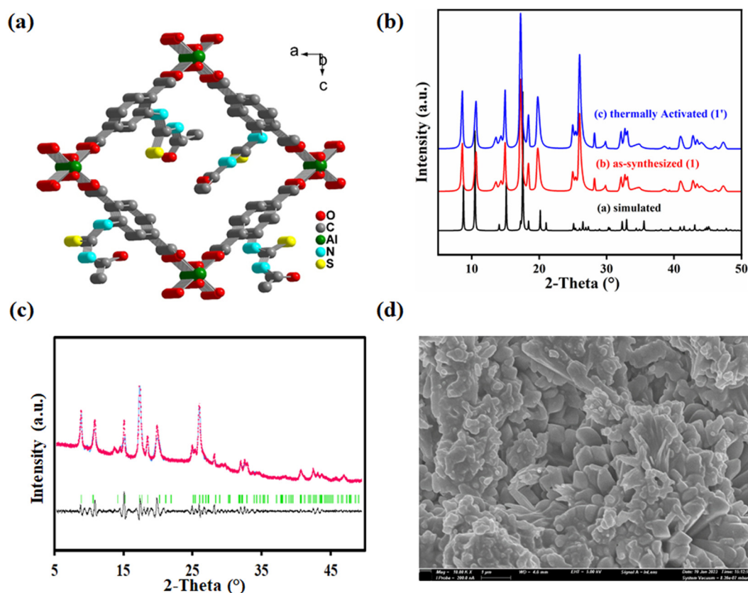
Fig. 1 (a) Simulated structure of 1. (b) PXRD profiles of 1 and 1' compared with simulated one. (c) Pawley refinement plot for the slow scan PXRD profile of 1' ( R_w and R_p are 5.4% and 3.8%, respectively). (d) FE-SEM image 1'.
