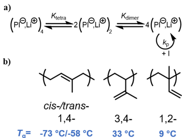
Scheme 1 (a) Aggregation equilibrium of polyisoprenyl lithium in non-polar solvents in analogy to Müller and Matyjaszewski; (b) possible microstructures of PI and their respective glass temperatures. 38,40
