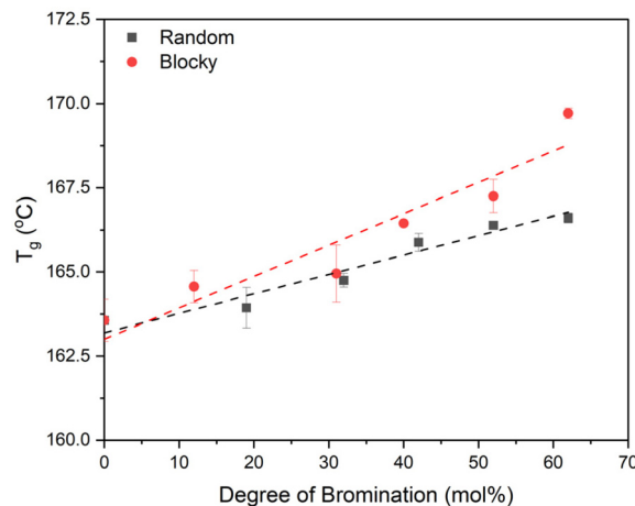
Fig. 9 Glass transition temperatures ( T_g ) of random (black squares) and blocky (red circles) amorphous BrPEKK determined from the midpoint of amorphous samples.
