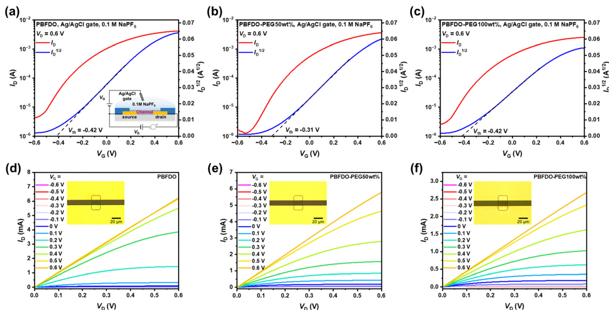
Fig. 4 Transfer (a)–(c) and output characteristics (d)–(f) of OEETs based on (a) and (d) PBFDO; (b) and (e) PBFDO-PEG50wt%; (c) and (f) PBFDO-PEG100wt%. The transfer characteristics were measured at V_{ds} = 0.6 V. The channel dimension used for this measurement is channel width/length = 20\ \mu\text{m}/10\ \mu\text{m} , while the thickness was around 70\ \text{nm} . Inset: Illustration of the OEET structure (a) and optical microscopic photos of the corresponding OEET channels (d)–(f).
