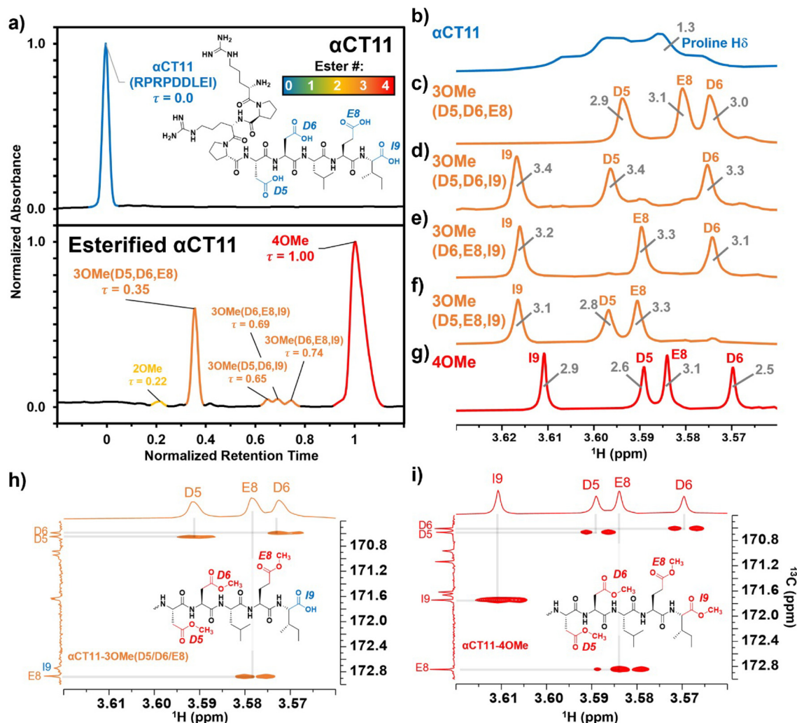
Fig. 1 Identifying the numbers and positions of methyl esters installed onto αCT11 through Fischer esterification. a) RP-HPLC of αCT11 (peak is blue), αCT11 with 2 methyl esters (peak is yellow), 4 different conformations of αCT11 with 3 esterified esters in either the D5, D6, E8, and/or I9 residues (αCT11-3OMe(D5,D6,E8, or I9), peaks are orange), and fully esterified αCT11, with 4 methyl esters (αCT11-4OMe, peaks are red). Retention time, and thus hydrophobic character, increased with the number of esters installed onto αCT11. The mobile phase consisted of water and acetonitrile (ACN), each with 0.1% v/v TFA, and each sample eluted between 23 and 26% ACN. Retention times were normalized to those of the αCT11 and αCT11-4OMe samples. 1 H NMR (800 MHz, DMSO-d 6 ) spectra of b) αCT11 (blue), c-f) each of the 4 αCT11-3OMe samples (orange), and g) αCT11-4OMe (red) methyl ester proton singlets (3.56–3.63 ppm) show which amino acids are esterified in each formulation. Integrals for each peak are plotted in gray on the spectra. Selective heteronuclear multiple bond correlation (selHMBC) of h) αCT11-3OMe(D5,D6,E8) (orange) and i) αCT11-4OMe (red) shows the most abundant -3OMe peak (-3OMe(A)) has esters installed on the D5, D6, and E8 positions, but not on the C-terminal I9.
