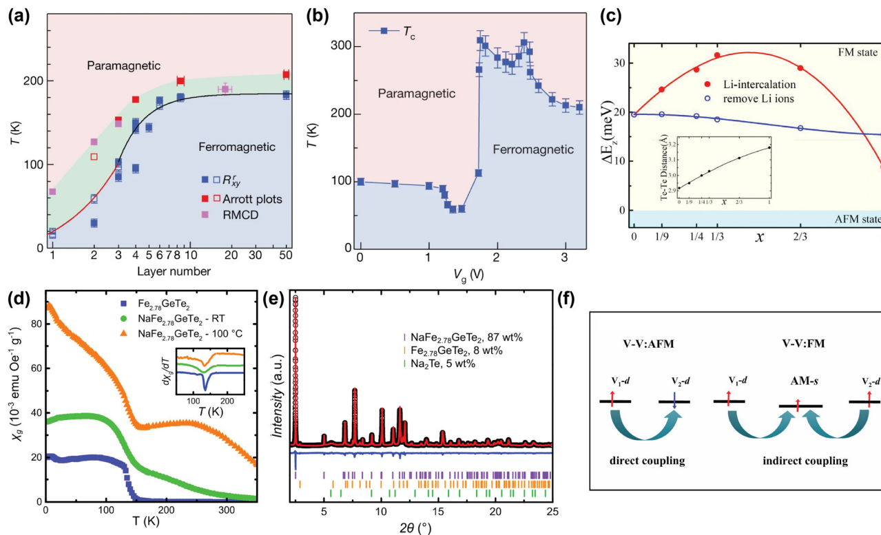
Fig. 2 (a) Magnetic phase diagram of \text{Fe}_3\text{GeTe}_2 as function of number of layer and temperature. T_C values determined from anomalous Hall measurements ( R_{xy}^r ), Arrott plots, and refractive magnetic circular dichroism (RMCD), are displayed in blue, red and magenta respectively. 58 (b) Magnetic phase diagram of trilayer \text{Fe}_3\text{GeTe}_2 flakes as function of gate voltage ( V_g ) and temperature. A higher V_g corresponds to a higher degree of Li intercalation. The T_C values were determined from temperature-dependent anomalous Hall measurements, extrapolated to zero. 58 (c) Calculated interlayer magnetic coupling energy ( \Delta E_z ) in \text{Li}_x\text{Fe}_3\text{GeTe}_2 bilayers as function of intercalation level x . The inset displays the calculated interlayer distance between the two interfacial Te sublayers. 95 (d) Temperature dependence of the specific magnetic susceptibility \chi_g of pristine \text{Fe}_{2.78}\text{GeTe}_2 (blue squares), Na-intercalated \text{Fe}_{2.78}\text{GeTe}_2 (green circles), and Na-intercalated \text{Fe}_{2.78}\text{GeTe}_2 annealed at 100 °C (orange triangles), measured at 0.01 T. The inset shows the derivative of \chi_g , indicating a T_C of ~140 K for all three samples. 96 (e) Rietveld refinement of \text{NaFe}_{2.78}\text{GeTe}_2 ( \lambda = 0.412852 Å), including reflections of unreacted \text{Fe}_{2.78}\text{GeTe}_2 (orange) and \text{Na}_2\text{Te} (green). 96 (f) Schematic plot of the change in the magnetic exchange mechanism from direct (left) to indirect (right) exchange, in alkali-intercalated \text{VS}_2 and \text{VSe}_2 . 97 Reproduced from ref. 97. Reproduced from ref. 58 with permission from Springer Nature, copyright 2018. Reprinted from ref. 95, with the permission of AIP Publishing, copyright 2021. Reprinted with permission from ref. 96. Copyright 2021 American Chemical Society.
