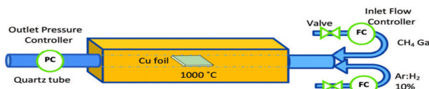
Fig. 17 Illustration of the chemical vapor deposition (CVD) to synthesize graphene. Reprinted with permission from ref. 106 Copyright 2021, Nature.
