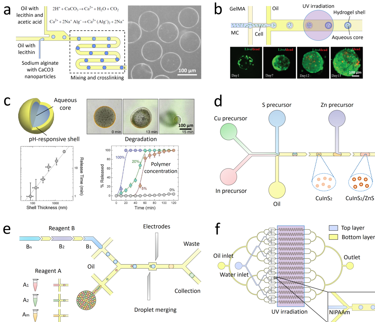
Fig. 2 Droplet-derived materials. a . When the droplets flow with acidic oil, \text{Ca}^{2+} ions are gradually released from \text{CaCO}_3 nanoparticles to crosslink the sodium alginate. 62 b . Microparticles with a core of methyl cellulose (MC) and a shell of GelMA are fabricated to encapsulate cells. After transfer into culture medium for further incubation, spherical cell aggregates are formed with high cell viability. 71 c . When a microcapsule is exposed to a trigger pH, its solid shell composed of pH-responsive polymers gradually degrades to release encapsulants. The release kinetics can be precisely controlled by the shell thickness, polymer concentration, and pH value. 72 d . Precursors of Cu, In, and S are compartmentalized into droplets and reacted to form \text{CuInS}_2 nanoparticles as the core. Then Zn precursors are injected into the droplets to form ZnS shells on the core particles. 73 e . A library of reagent A is compartmentalized into droplets and reinjected into the channel. Another library of reagent B, spaced by an oil phase, is successively introduced into the channel and compartmentalized into droplets. The two sets of droplets are merged in pairs, producing a library of different combinations. The synthesized products are driven into the collection channel by negative pressure, while the spacing oil between reagent B flows into the waste channel. 74 f . Droplets of N -isopropylacrylamide (NIPAAm) are generated and polymerized in 16 channels in parallel to achieve mass production of microparticles. 75 Panel A is adapted with permission from ref. 62. Copyright (2007) WILEY-VCH Verlag GmbH & Co. KGaA, Weinheim. Panel B is adapted with permission from ref. 71. Copyright (2019) WILEY-VCH Verlag GmbH & Co. KGaA, Weinheim. Panel C is adapted with permission from ref. 72. Copyright (2013) American Chemical Society.
