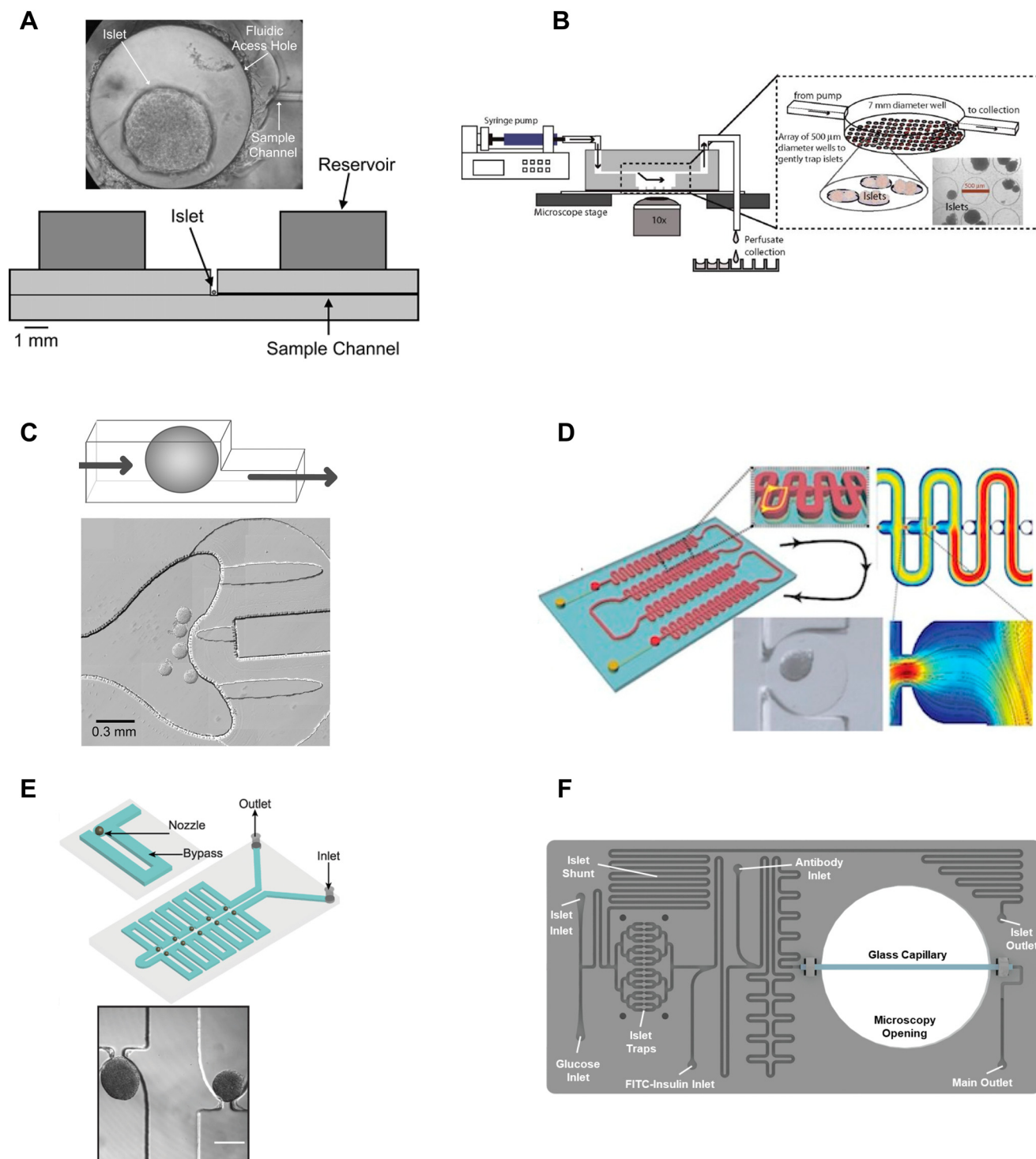
Fig. 1 Immobilization methods used in microfluidic devices for islet entrapment. A ) Open chamber loaded with a single islet for insulin secretion using capillary electrophoresis. Reprinted (adapted) with permission from ref. 17. Copyright 2003 American Chemical Society. B ) Closed chamber device with an array of 500 \mu\text{m} wells to capture islets for simultaneous measurement of \text{Ca}^{2+} -influx/mitochondrial membrane potential and insulin secretion. Reproduced with permission from ref. 27. C ) A dam-wall device that holds islets up against a wall using controlled flow for enhanced media flow through the tissue. © 2011 Sankar et al. Reproduced with permission from ref. 19 and 30. D ) A microfluidic device with an array of hydrodynamic traps to trap microencapsulated islets to explore hypoxia. Reprinted (adapted) with permission from ref. 34. Copyright 2013 American Chemical Society. E ) A microfluidic device with 10 hydrodynamic traps and associated bypass in series to consecutively capture loaded islets. Reproduced with permission from ref. 31. F ) A microfluidic device with 16 hydrodynamic traps in parallel with automated islet loading, stimulating and insulin secretion sensing. Reproduced with permission from ref. 36.
