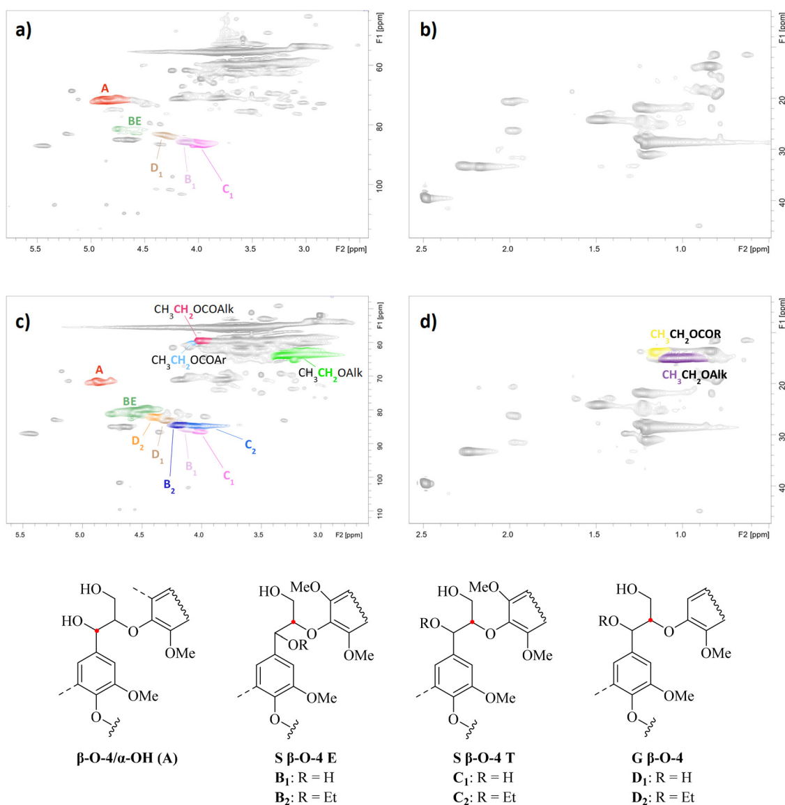
Fig. 3 2D HSQC spectra of ethanol extracted lignin (EEL; a and b) and reactive extracted lignin (REL; c and d). Reaction conditions to produce REL: t = 4 h, [EtOH] = 99%, [H 2 SO 4 ] = 0.15 M, T = \text{reflux} .
