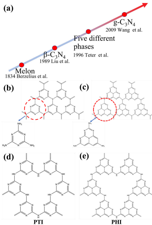
Fig. 1 (a) The roadmap of the development of carbon nitrides. (b) Triazine and (c) tri- s -triazine (heptazine) structures of g-C 3 N 4 . (d) Structures of poly(triazine imide) (PTI) and (e) poly(heptazine imide) (PHI).
