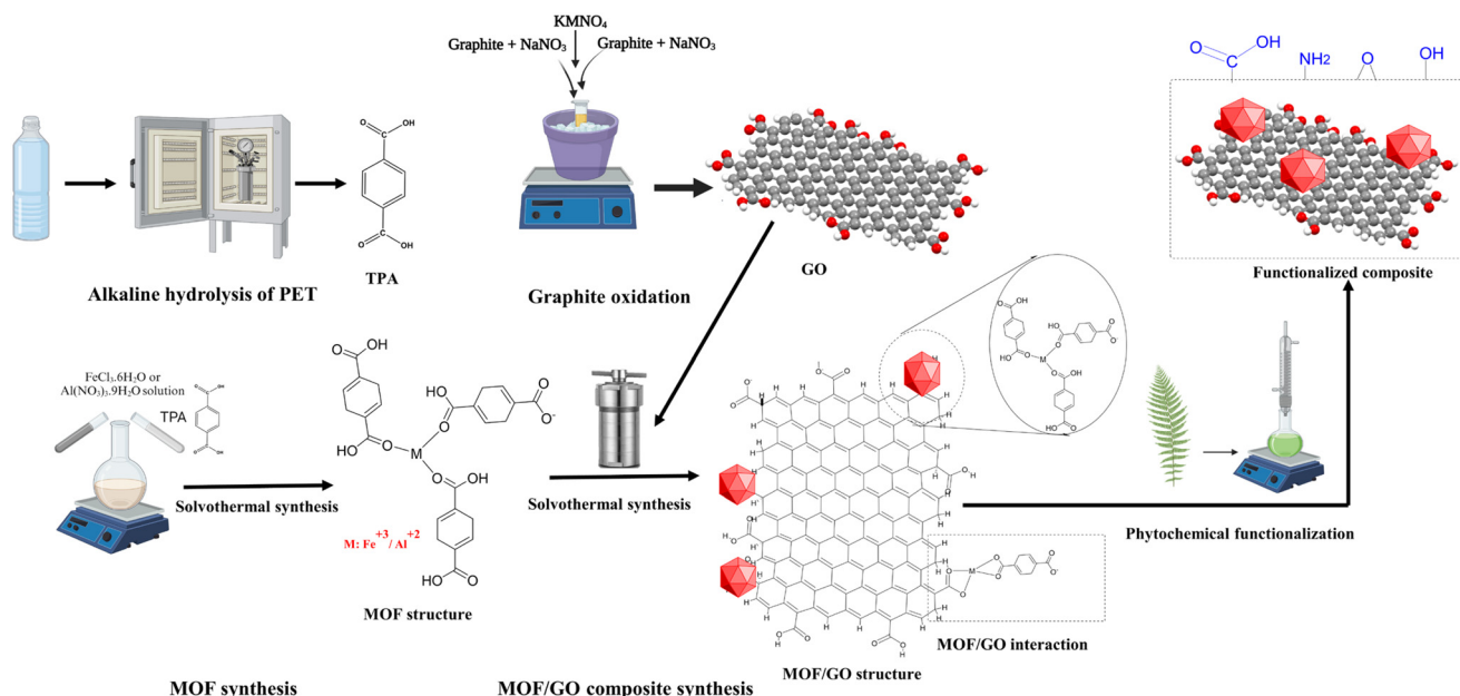
Fig. 1 Synthesis of the phytochemically functionalized GO/MOF composite.
