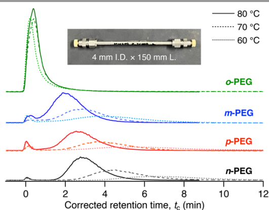
Fig. 2. HPLC chromatograms for o -PEG (green), m -PEG (blue), p -PEG (red), and n -PEG (black) on the 1 -packed column using DMF as the eluent at 80 °C (solid line), 70 °C (dashed line), and 60 °C (dotted line). The inset is a photograph of the 1 -packed column, demonstrating the dimensions. t_c denotes the corrected retention time, t_c = t_R - t_0 , where t_R is the retention time and t_0 is the column hold-up time. For more detailed measurement conditions, see ESI. A small front peak near t_0 is considered a breakthrough peak, which is occasionally observed in LC under certain conditions (see Fig. S4 in ESI) 35,36 .
