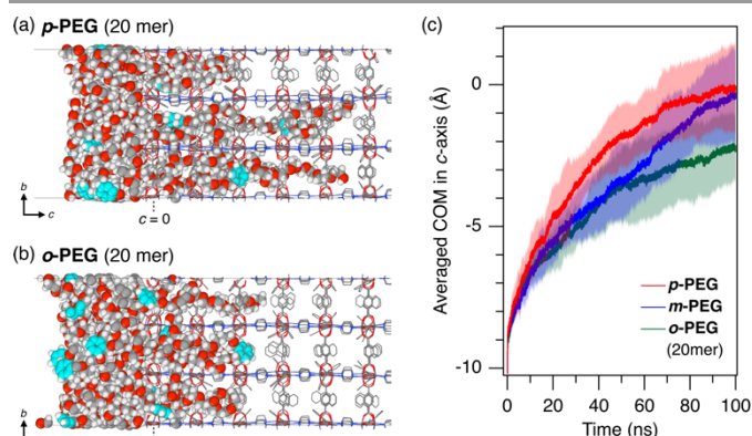
Fig. 4. Representative MD snapshots of (a) p -PEG and (b) o -PEG after 100-ns infiltration from the ab surface of 1 at 393 K; shortened versions of the PEGs were used (20 mer). For more detailed simulation conditions, see ESI. The framework of 1 and PEGs are depicted using wireframes and space-filling models, respectively. Hydrogen atoms of the framework are omitted for clarity. Xylene unit in the PEG chain is coloured aqua blue. (c) Time evolution of the averaged COM of p -PEG (red), m -PEG (blue), and o -PEG (green) in the c -axis of 1 . The origin ( c = 0 ) is defined as the COM of Zn dimers of the paddle wheel cluster at the PEG/ 1 interface. Averaged data from the five MD simulation runs are plotted as solid lines with shaded error bands of \sigma ( N = 5 ).
