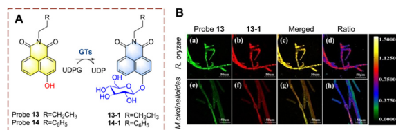
Fig. 11 (A) The structure and response mechanism of probe 13 and probe 14. (B) Confocal microscopy images of probe 13 (50 \mu M, 8 h) and 13-1 in R. oryzae and M. circinelloides (reprinted with permission from ref. 43 Copyright © 2018, American Chemical Society).
