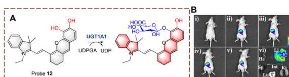
Fig. 10 (A) The structure and response mechanism of probe 12. (B) Image of probe 12 (10 \mu M, 0–30 min) in mice and isolated organs (reprinted with permission from ref. 42 Copyright © 2021, John Wiley and Sons).
