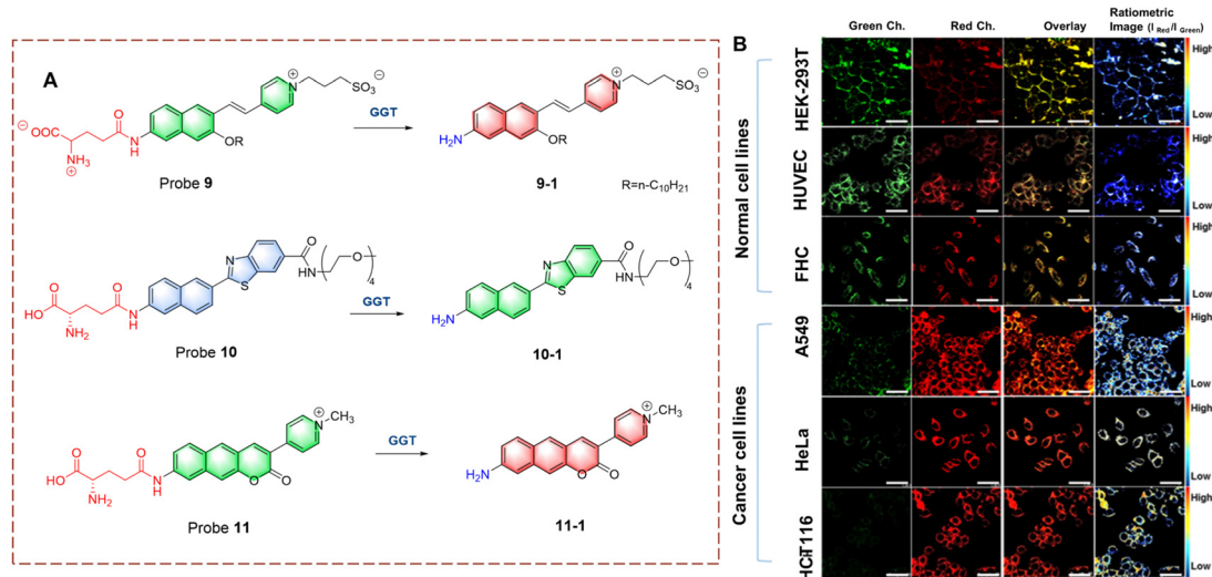
Fig. 9 (A) The structure and response mechanism of probe 9, probe 10 and probe 11. (B) Fluorescence images of normal cell lines and cancer cell lines with probe 9 (5.0 \mu M) (reprinted with permission from ref. 34 Copyright © 2020, American Chemical Society).
