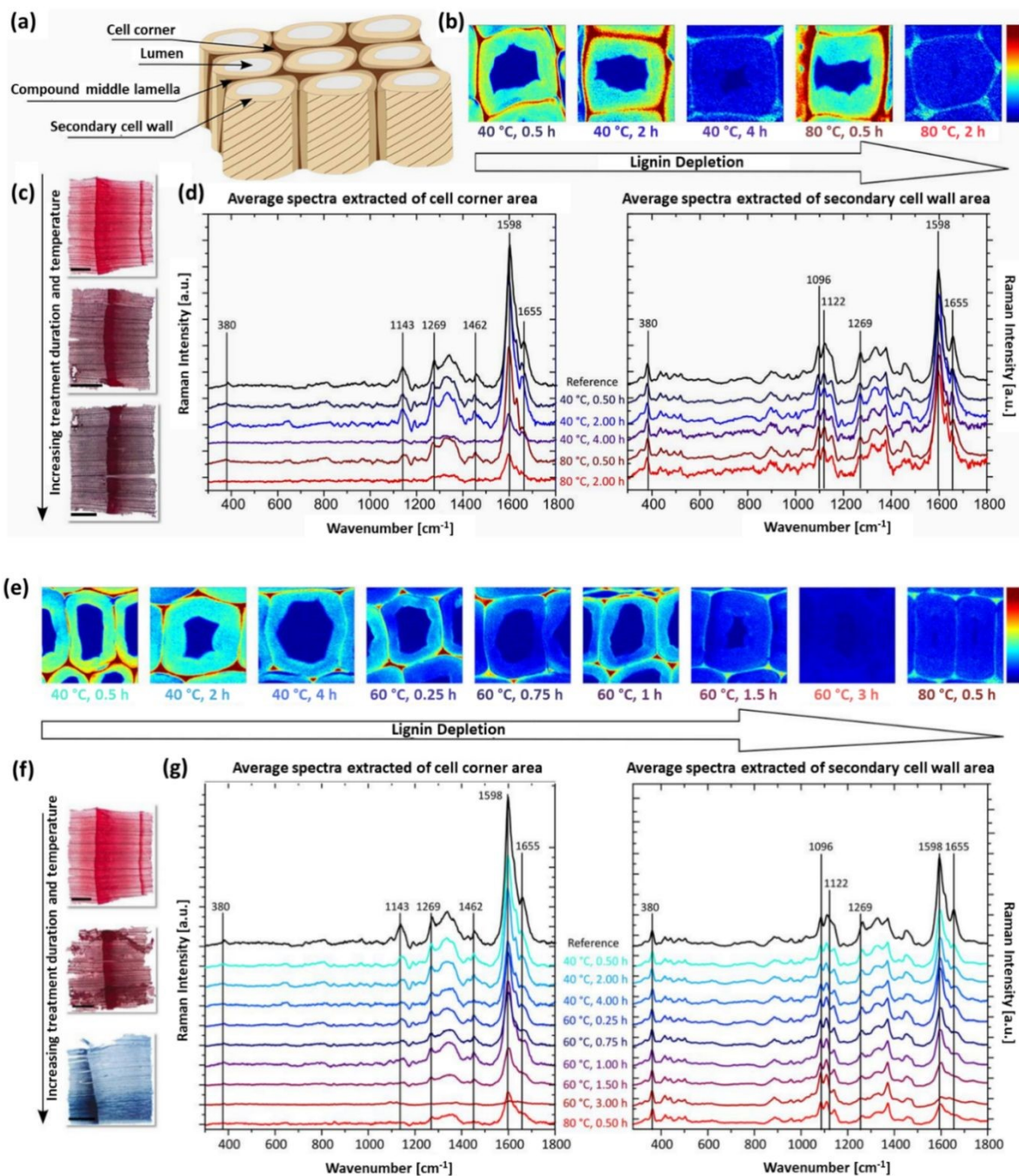
Fig. 11. Cross-sections characterization of soda-pulped and acid-bleached spruce wood. (a) Schematic representation of a wood tissue model composed of various anatomical regions, Raman images based on the integration of the main lignin band at 1598 \text{cm}^{-1} obtained from various regions for (b) soda-pulped and (e) acid-bleached samples. Cross-sectional images of stained spruce wood samples utilizing safranin red and methylene blue, which resulted in cellulose appearing blue, whereas lignified tissue took on a red hue after (c) alkaline and (f) acid treatment. Calculated average Raman spectra extracted from the secondary cell wall region and cell corner area (normalized on the band at 380 \text{cm}^{-1} ) after (d) soda pulping and (g) acid bleaching methods. (Reproduced from Ref. 157 with permission from MDPI. Copyright 2018)
