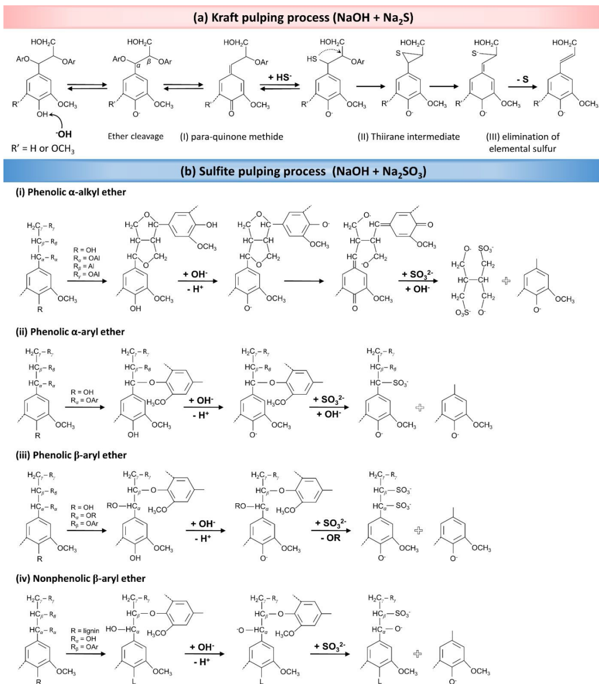
Fig. 6. The delignification mechanism during pulping processes. (a) Wood pulping reactions in the presence of an alkaline solution of Na 2 S (Kraft pulping). (Reproduced from Ref. 66 with permission from WILEY-VCH Verlag GmbH & Co. Copyright 2020). (b) The mechanism for partial in situ lignin removal in a solution containing NaOH and Na 2 SO 3 (sulfite pulping process). (Reproduced from Ref. 68 with permission from the American Chemical Society. Copyright 2021)
