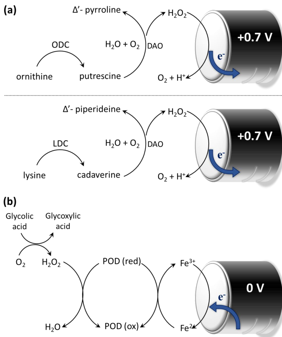
Fig. 37. Enzymatic mechanisms in (a) the legume cotyledon tissue biosensors (Reproduced from Ref. 285 with permission from Elsevier, Copyright 1993) and (b) ferrocene-mediated spinach tissue-based biosensor. (Reproduced from Ref. 293 with permission from Elsevier, Copyright 1994)
