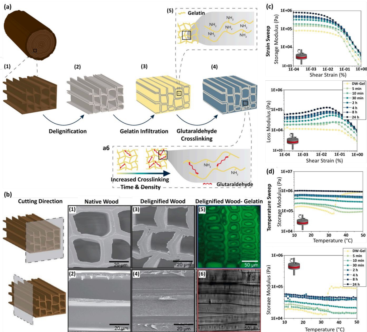
Fig. 25. (a) Manufacturing process of the cross-linked DW-gelatin composite (DW-Gel): (a1) native wood, (a2) DW, (a3) infiltration with gelatin, and (a4) additional cross-linking in an aqueous glutaraldehyde solution. (a5) Gelatin protein chains with lysine residues and free amino groups integrated into the DW structures. (a6) Tuning the cross-linking degrees of gelatin protein chains by adjusting cross-linking time in the glutaraldehyde solution. (b) SEM images of (b1,b2) the cross-section and longitudinal-tangential surface of native spruce and (b3,b4) the cross-section and longitudinal-tangential surface of delignified spruce. (b5,b6) Confocal fluorescence microscopy and phase contrast images of the DW-Gel cross-section, respectively. (c) Storage and loss modulus versus shear strain. (d) Temperature-dependent storage and loss modulus in different groups. (Reproduced from Ref. 215 with permission from Elsevier, Copyright 2023).
