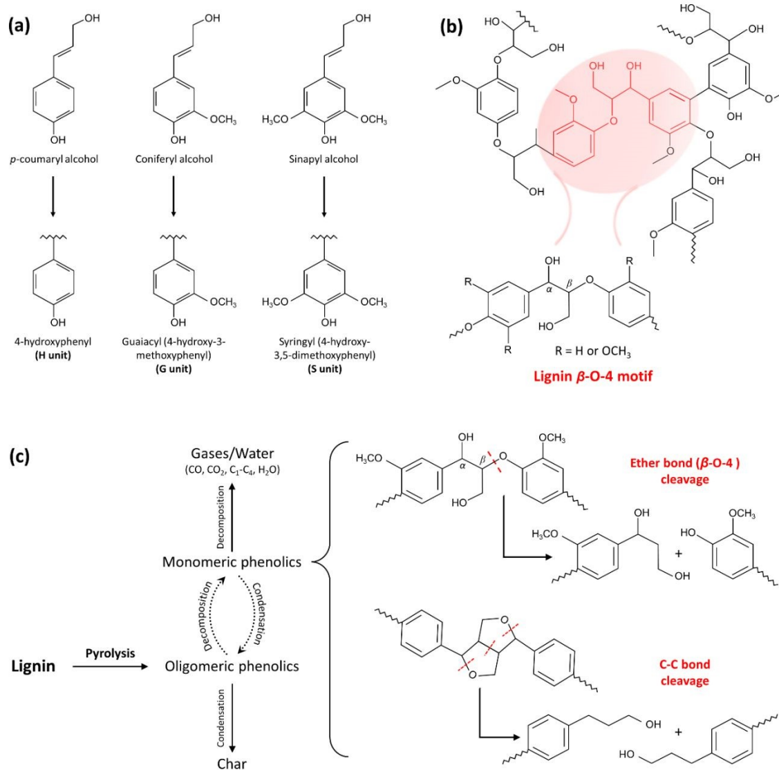
Fig. 3. The chemical structures of lignin and its pyrolysis products. (a) Chemical structures of lignin monolignols composed of p -coumaryl alcohol, coniferyl alcohol, and sinapyl alcohol that contribute to the formation of three main
