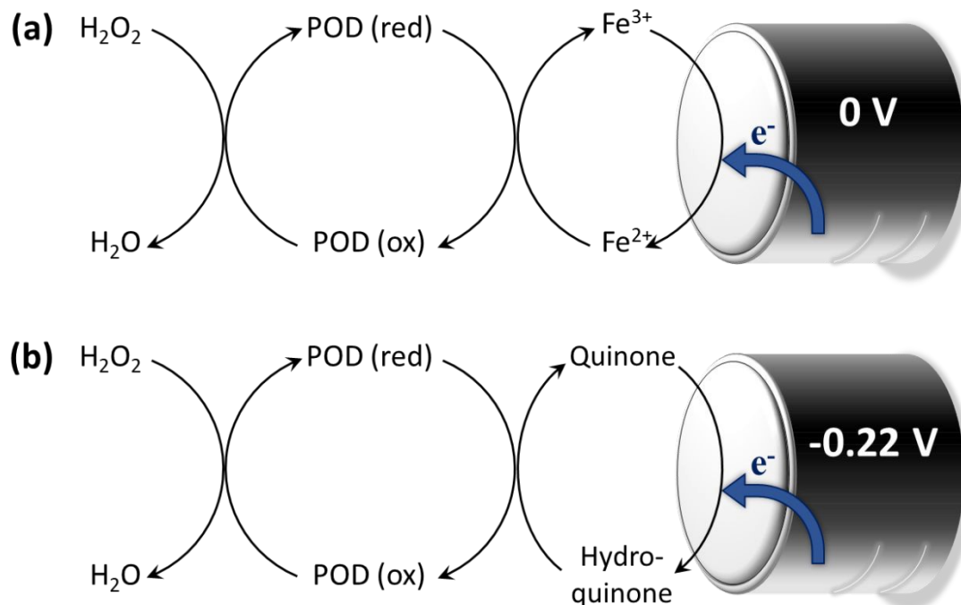
Fig. 36. Enzymatic processes of hydrogen peroxide reduction in (a) ferrocene-mediated (Reproduced from Ref. 274 with permission from Elsevier , Copyright 2001) and (b) quinone-mediated peroxidase catalysis. (Reproduced from Ref. 275 with permission from Elsevier , Copyright 2000)
