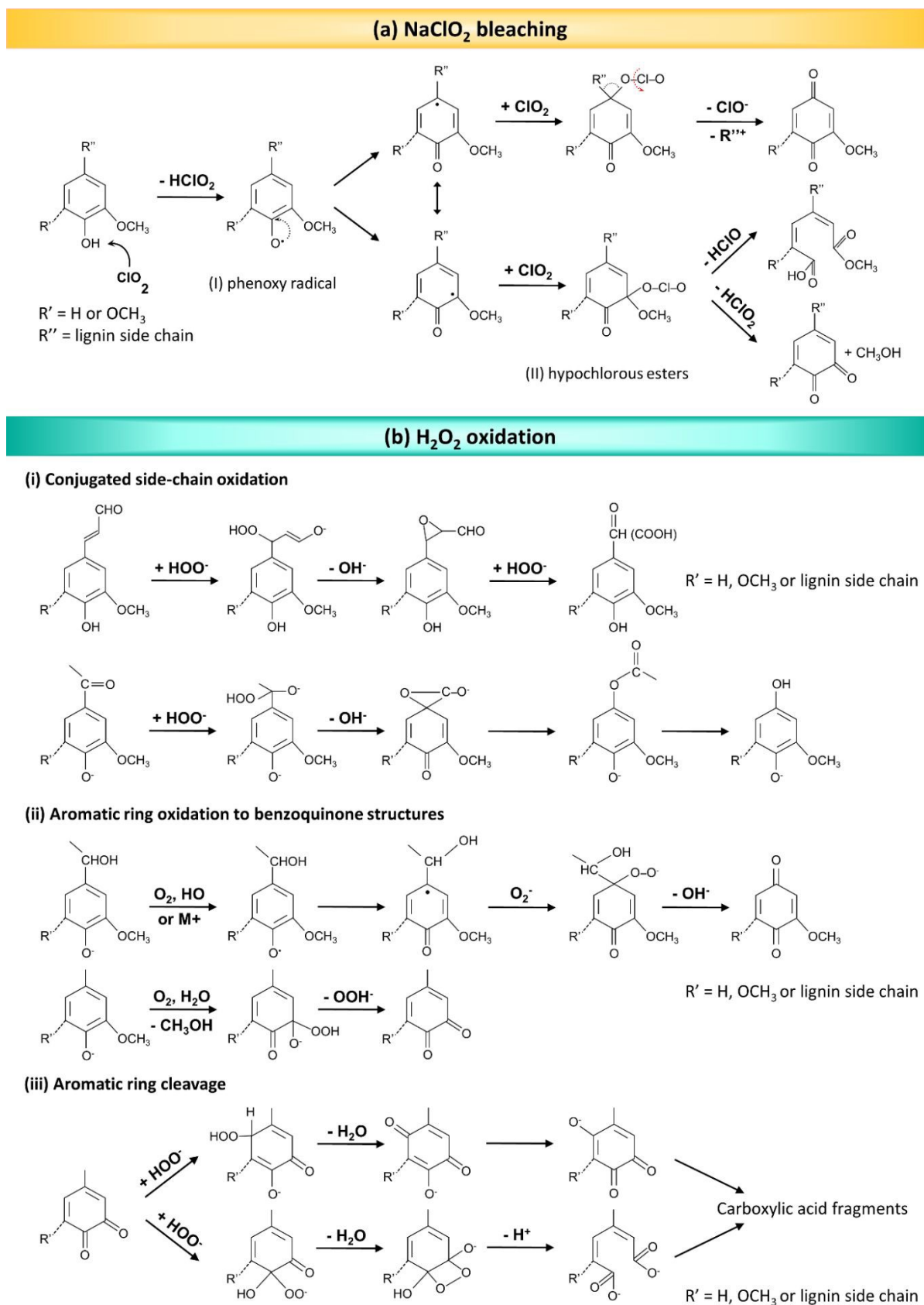
Fig. 7. The delignification mechanism during bleaching processes. (a) The lignin oxidation mechanism by ClO 2 .
