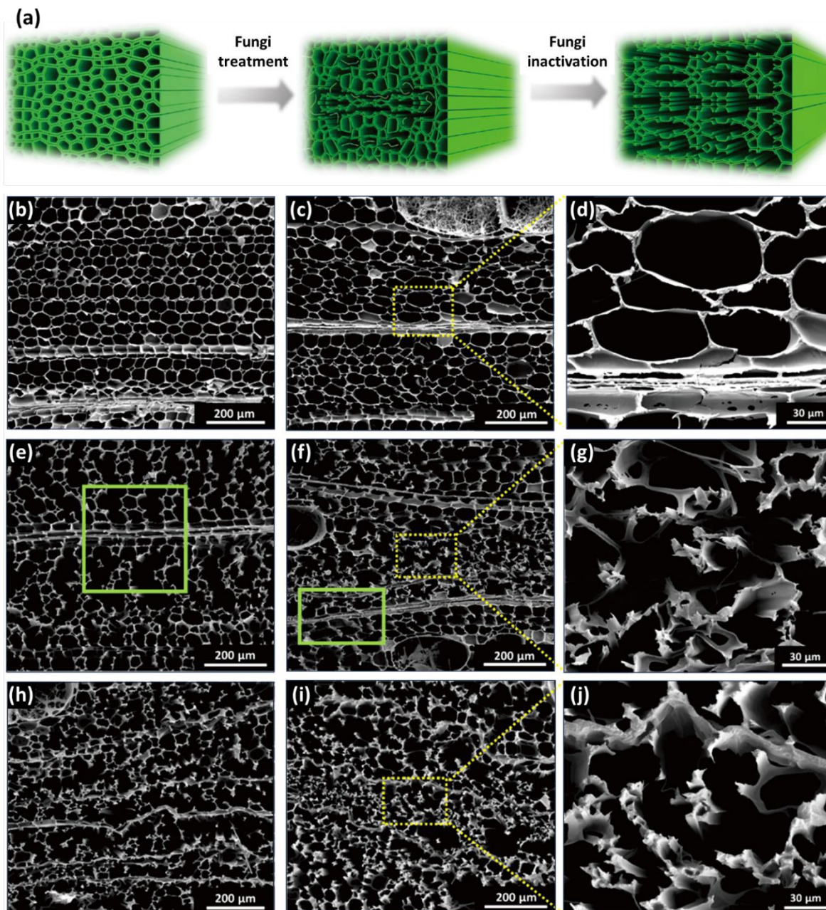
Fig. 4. Morphological changes in balsa wood decaying after exposure to G. applanatum fungus. (a) Schematic representation of the transformation of the wood structure during fungal treatment. (b) SEM images at different magnifications obtained from native balsa (0% weight loss). (c and d) Balsa wood after 4 weeks of exposure (15% weight loss). (e) Balsa wood after 6 weeks of exposure (25% weight loss). (f and g) Balsa wood after 8 weeks of exposure (35% weight loss). (h) Balsa wood after 10 weeks of exposure (45% weight loss). (i and j) Balsa wood after 12 weeks of exposure (55% weight loss). (Reproduced from Ref. 110 with permission from Science . Copyright 2021).
