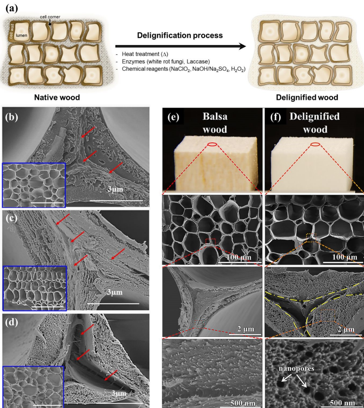
Fig. 14. The effect of delignification on the porosity and surface area of DW samples. (a) Schematic representation of lignin removal from cell wall causing a significant decrease in density. Comparative SEM images of (b) native balsa wood, (c) lignin-modified wood in alkaline- \text{H}_2\text{O}_2 media, and (d) \text{NaClO}_2 -based delignified balsa wood. (Reproduced from Ref. 85 with permission from WILEY-VCH Verlag GmbH & Co. Copyright 2017). Low- and high-magnification SEM images of (e) native balsa wood and (f) DW with nanopores indicated by arrows. (Reproduced from Ref. 77 with permission from the American Chemical Society. Copyright 2018).
