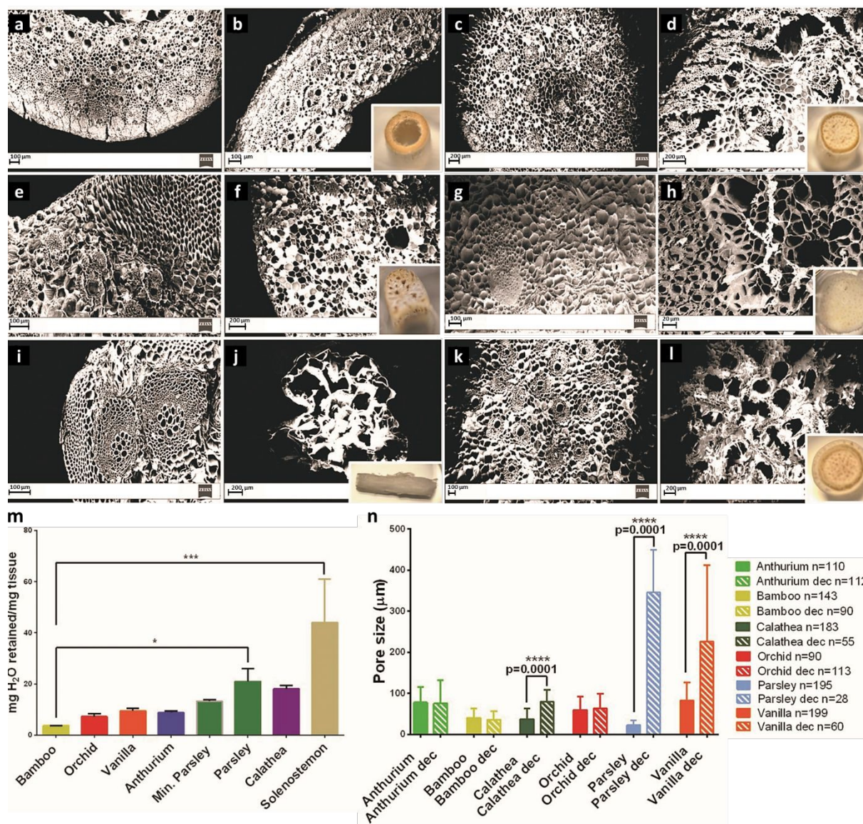
Fig. 13. Pore size and distribution profiles of various plant tissues after decellularization. SEM images of plant tissues before (left panel) and after (right panel) decellularization for: (a, b) bamboo, (c, d) Anthurium warocqueanum , (e, f) Calathea zebrina , (g, h) orchid pseudobulb, (i, j) parsley, and (k, l) vanilla. (m) The normalized water mass retained in each stem ( n = 4 , *p < 0.05 and ***p < 0.001 ). (n) and (n) comparison of average pore sizes of stems pre- and post-decellularization ( p < 0.05 ). (Reproduced from Ref. 27 with permission from WILEY-VCH Verlag GmbH & Co. Copyright 2017).
